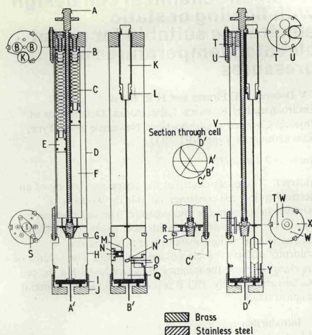
Figure 1 Sectional diagram of cell container: A, gear; B, PTFE end plug; C, steel spring; D, reservoir unit body; E, PTFE piston; F, electrolyte reservoir; G, PTFE tube inset; H, cell unit body; I, pH electrode; J, brass cap; K, PTFE pressure-sensitive bag; L, viton O ring; M, PTFE F05 sinter; N, N', silver-silver chloride electrode; O, PTFE electrode holder; P, electrode seal; Q, cell compartment; R, valve, EN58J; S, valve liner, EN58J; T, locating pin; U, brass studding; V, drive shaft; W, electrolyte entry port; X, electrolyte exit port; Y, push-in PTFE liner
